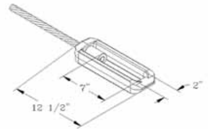
SWIVEL CABLE END
