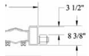
HOIST FRAME DETAIL
