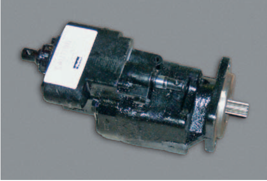
Pump/Valve combination
